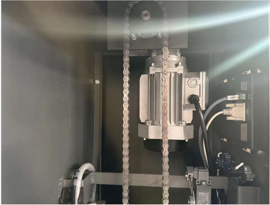
Service detail | Internal drive and chain arrangement
